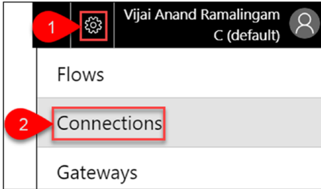
Figure 5-8. Connections
