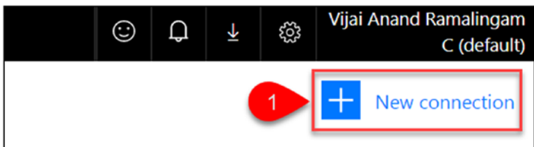
Figure 5-3. New connection
