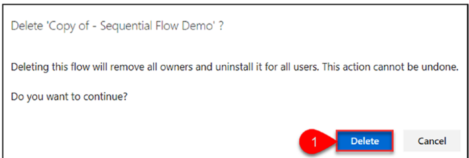
Figure 6-10. Confirm deletion
