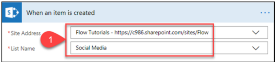
Figure 2-104. Action parameters
