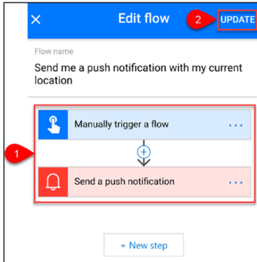
Figure 4-28. Flow details
