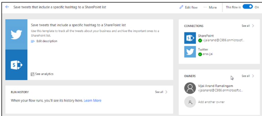
Figure 2-10. Flow details
