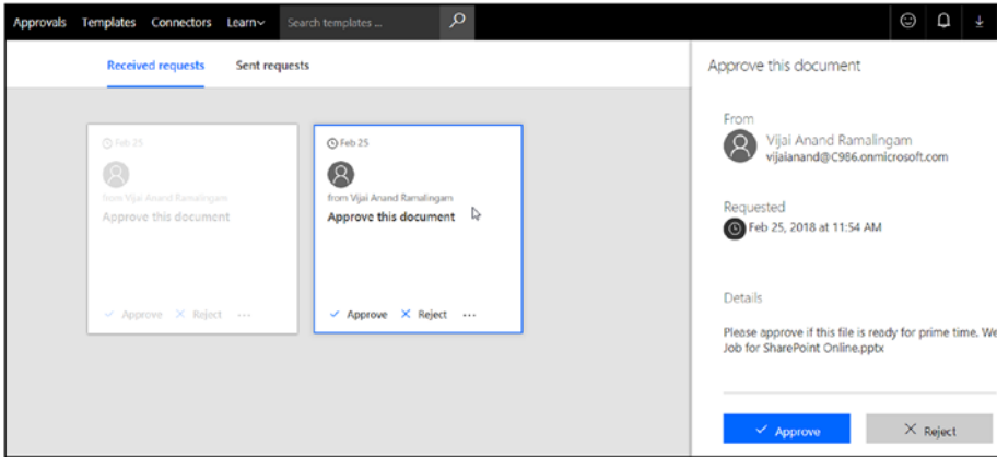
Figure 3-1. Received requests
