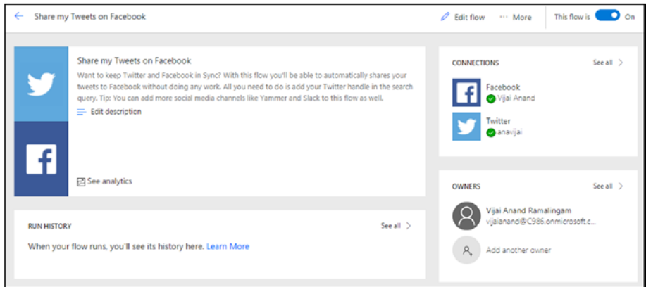
Figure 1-30. Flow details
