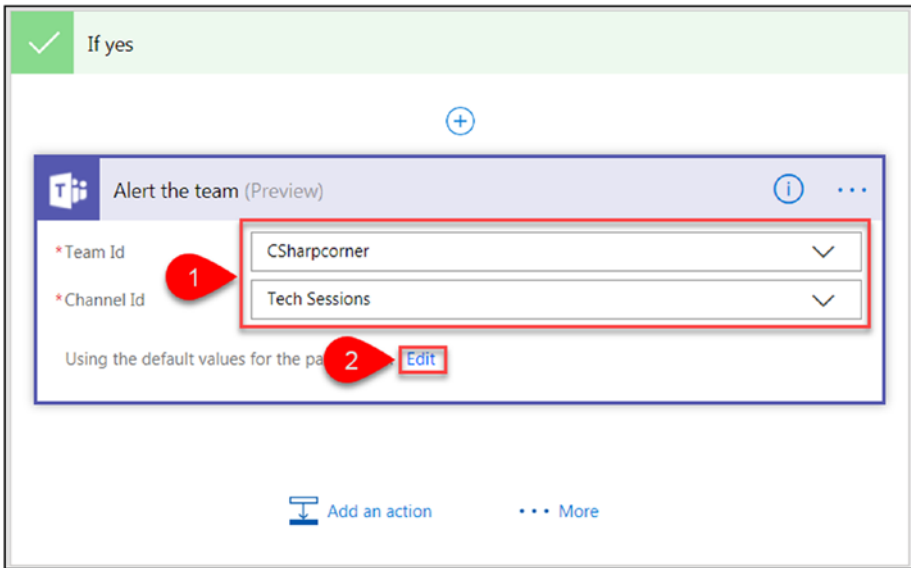
Figure 2-78. Action parameters
