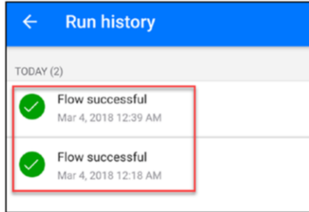
Figure 4-31. Run history
