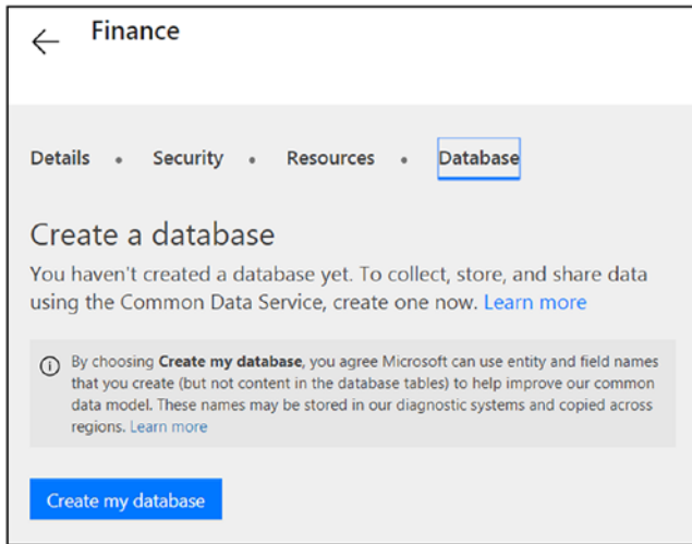
Figure 6-44. Environment database
