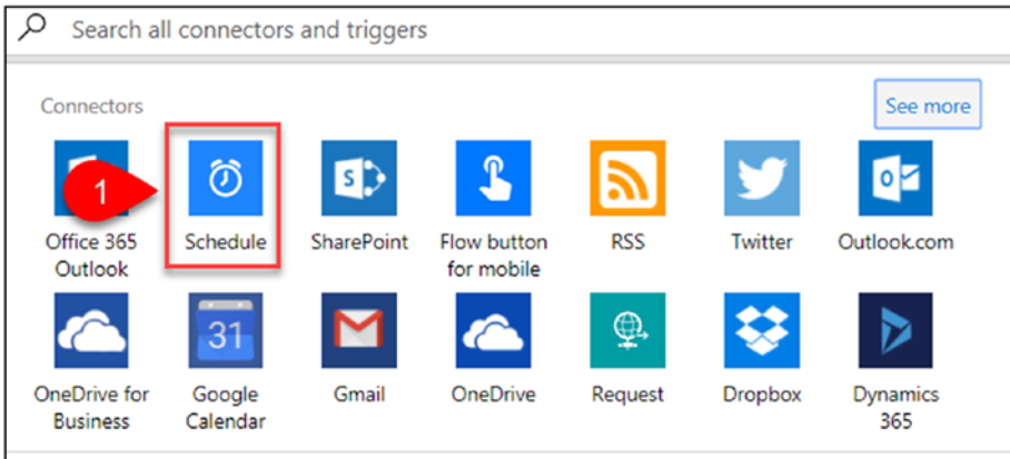
Figure 2-85. Schedule connector
