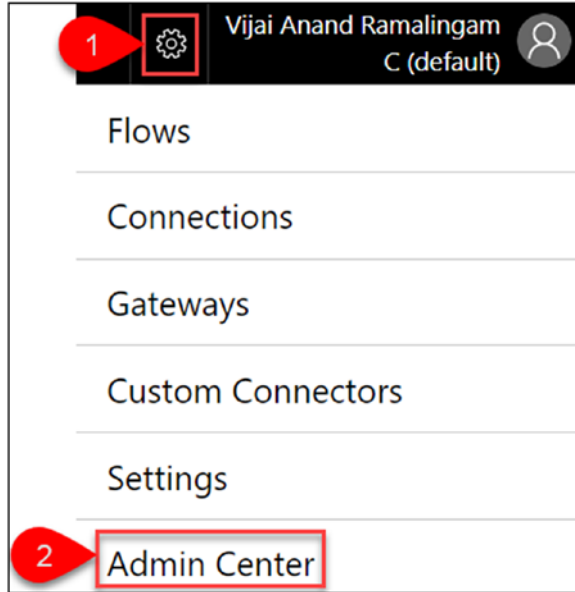
Figure 6-46. Admin Center
