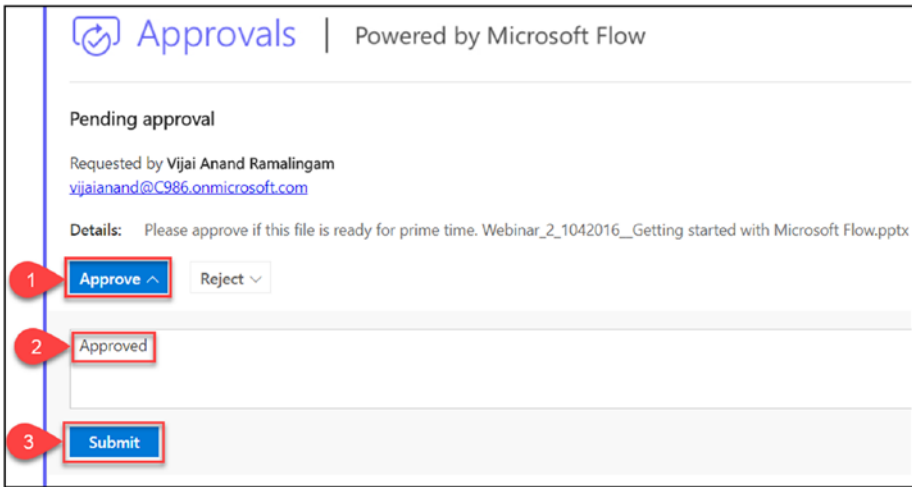
Figure 3-24. Approval email
