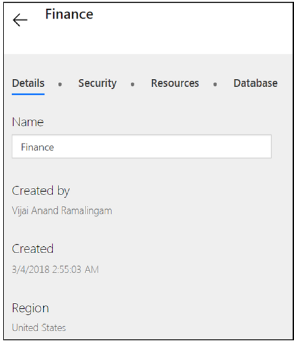
Figure 6-40. Environment details
