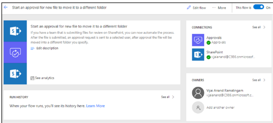
Figure 3-22. Flow details
