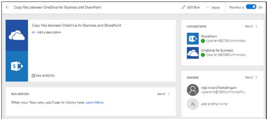
Figure 2-66. Flow details
