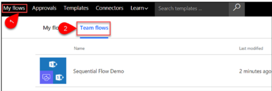
Figure 6-13. Team flows
