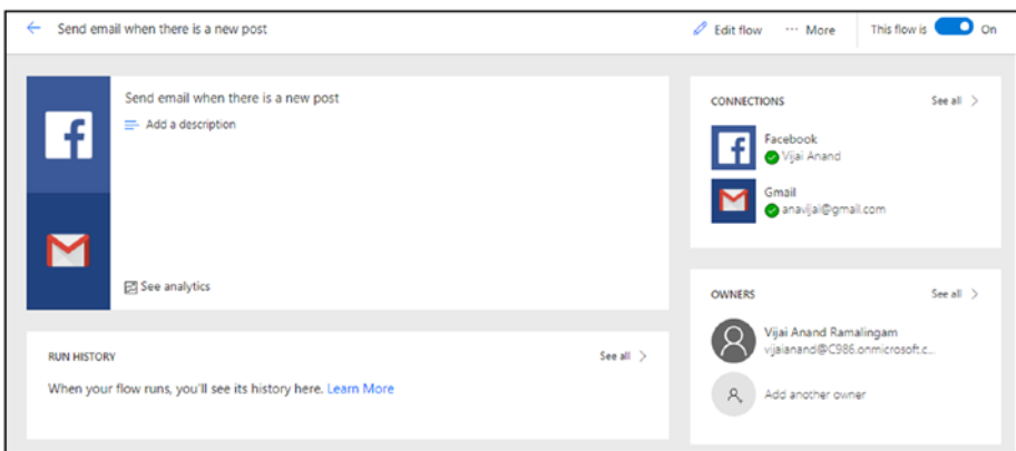
Figure 1-42. Flow details
