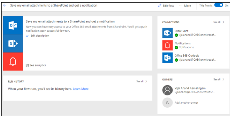
Figure 2-22. Flow details
