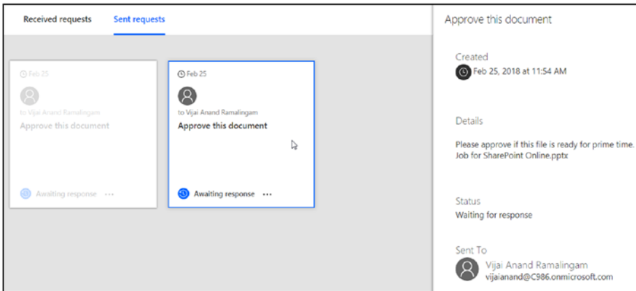
Figure 3-2. Approved requests
