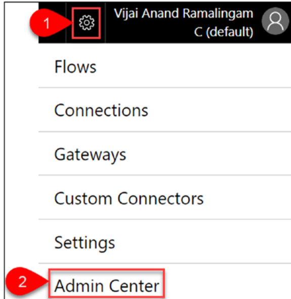
Figure 6-38. Admin Center
