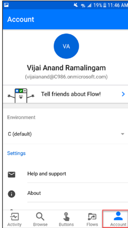
Figure 4-7. Account details
