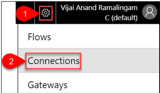
Figure 5-1. Connections
