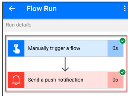
Figure 4-32. Run details
