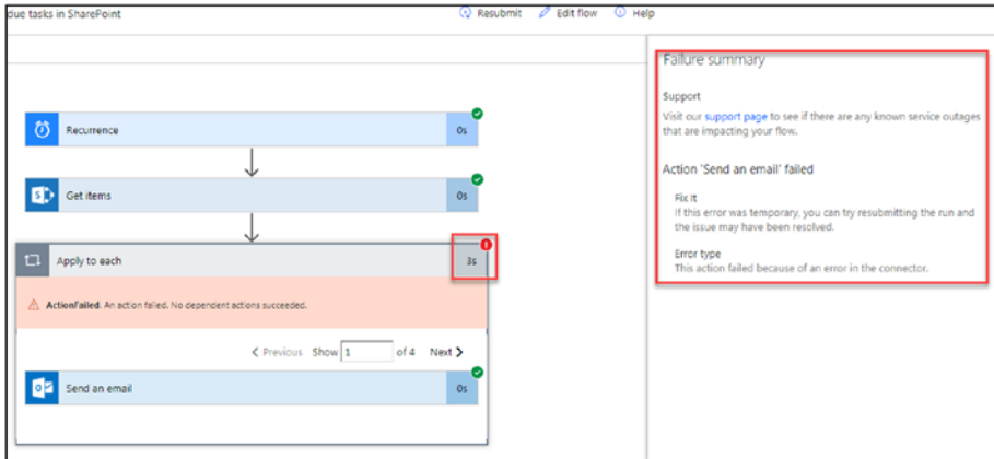
Figure 6-31. Failure summary
