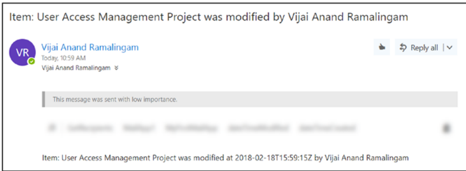
Figure 2-34. Received email
