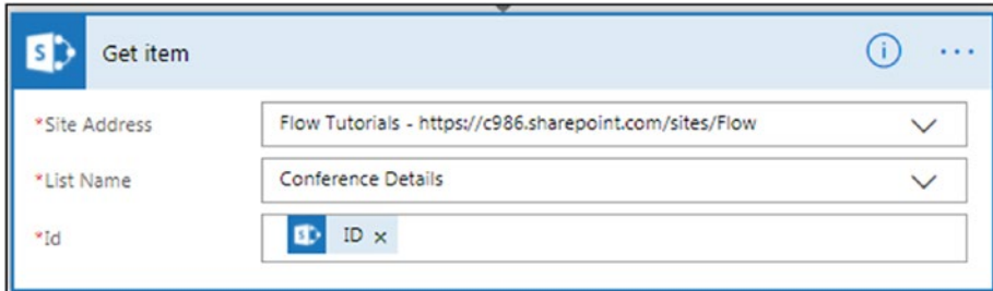
Figure 2-50. Action parameters
