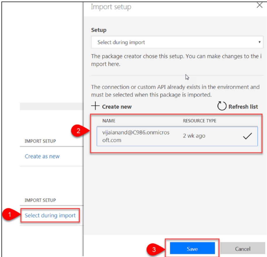
Figure 6-22. Import setup
