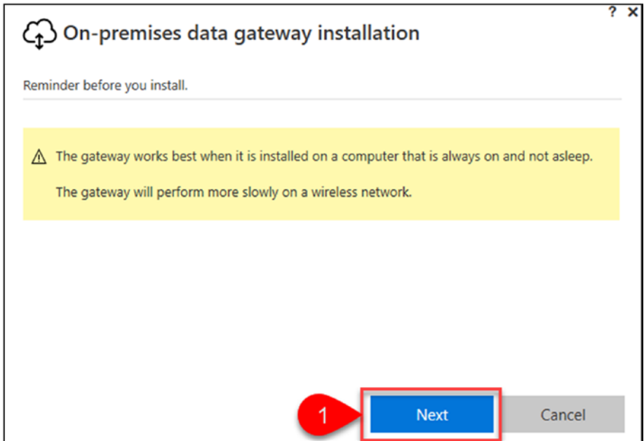
Figure 5-22. Reminders
