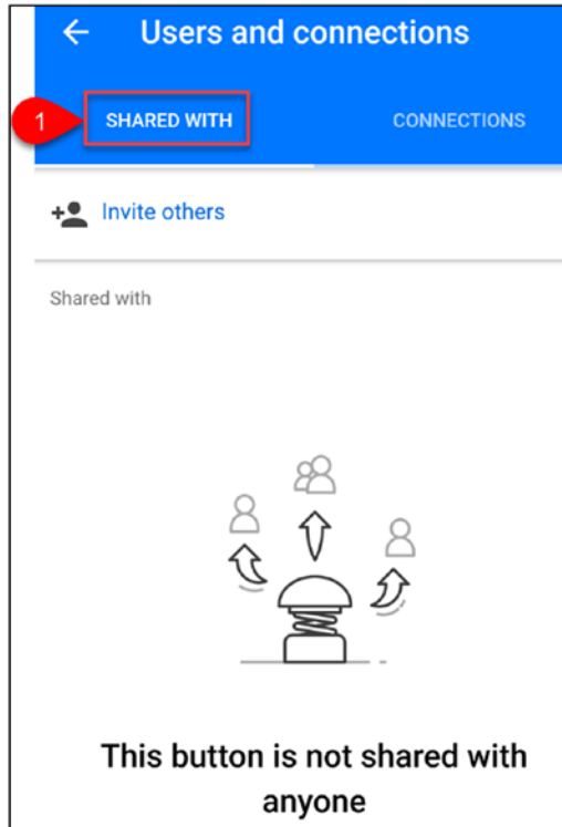
Figure 4-29. Manage users
