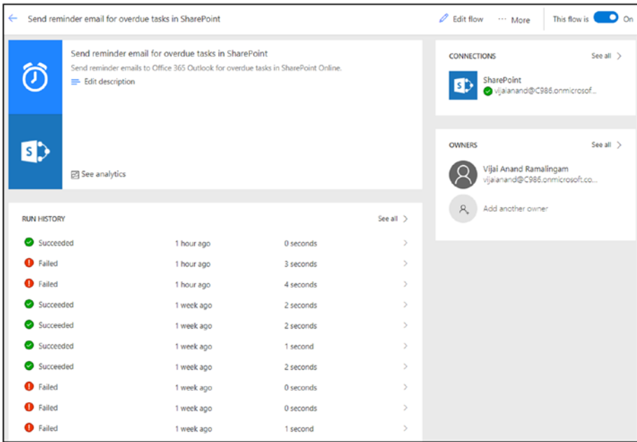
Figure 6-27. Flow details
