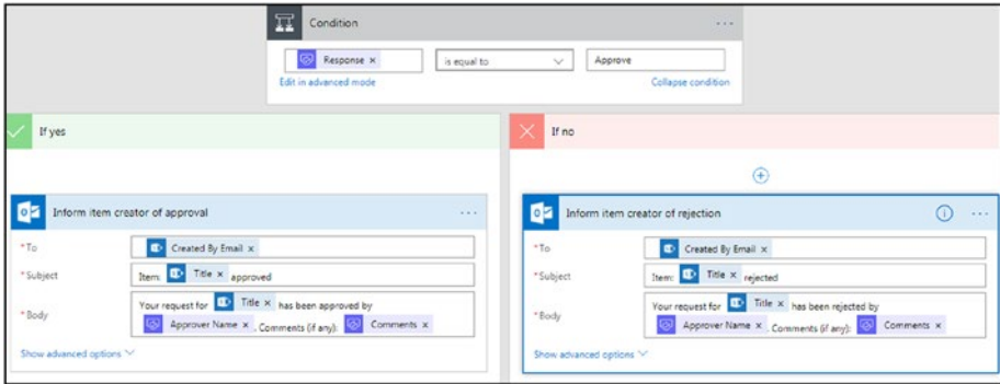
Figure 3-7. Conditions
