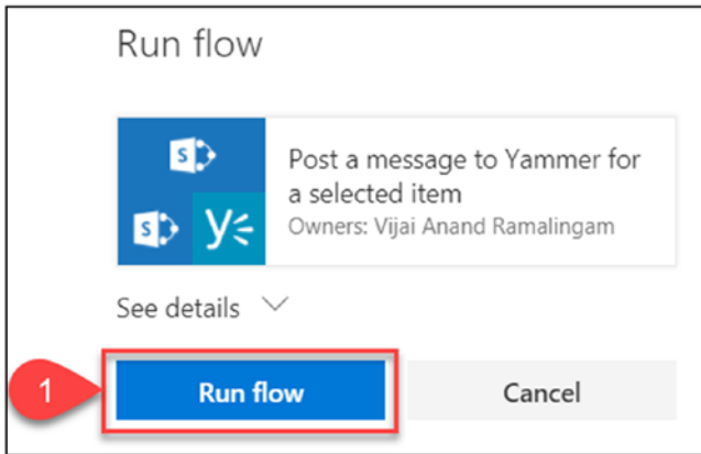
Figure 2-58. Run flow
