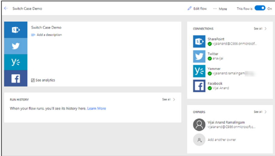
Figure 2-118. Flow details
