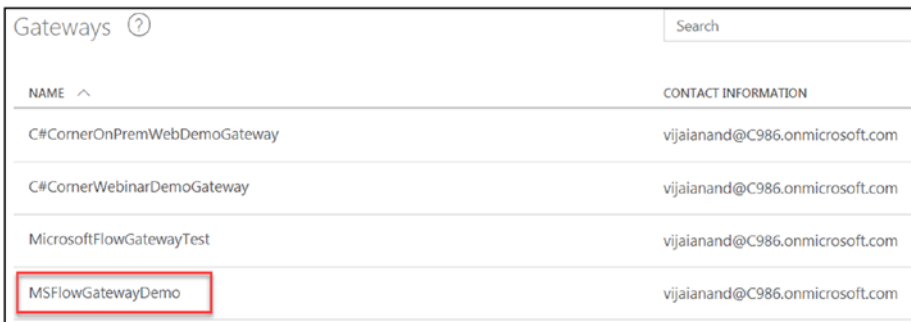
Figure 5-30. Creation success
