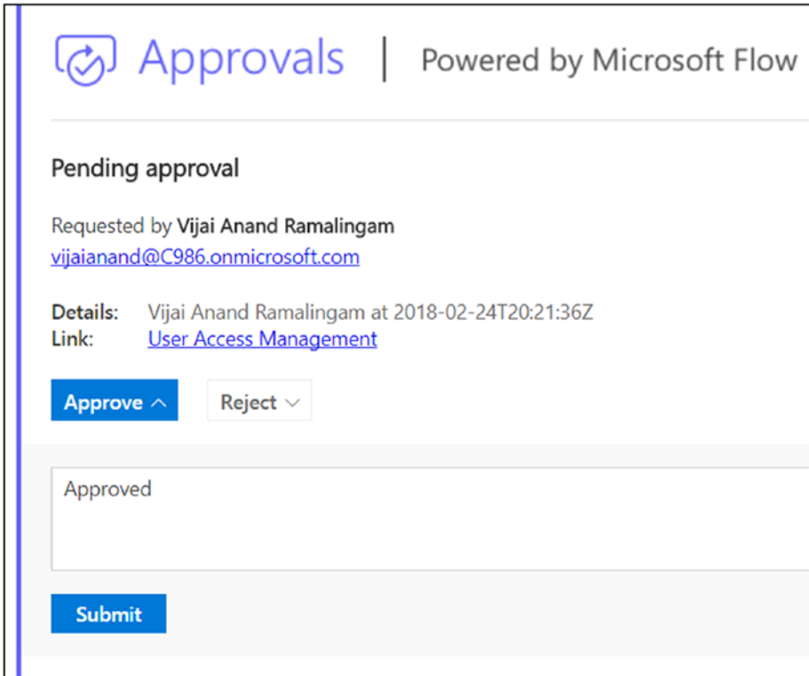
Figure 3-12. Approval email
