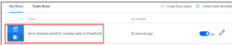
Figure 6-25. Imported flow
