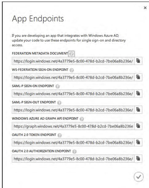
FIGURE 5-3 A list of protocol endpoints for an Azure AD tenant
