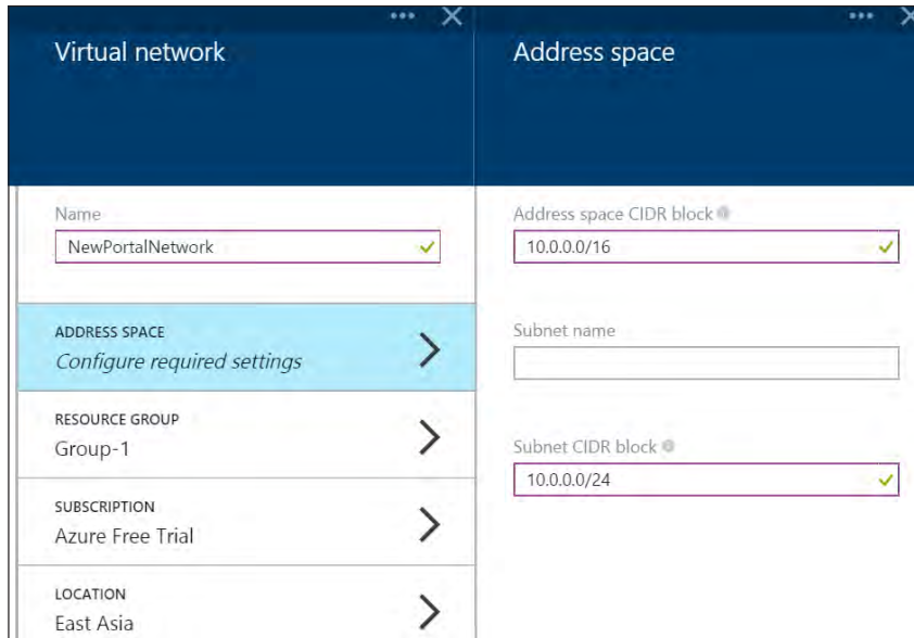
FIGURE 5-9 Creating a new virtual network
