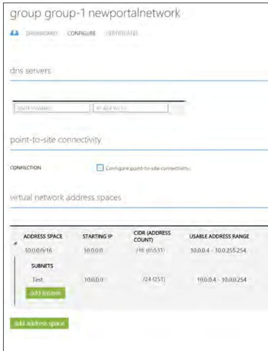
FIGURE 5-12 Editing subnet settings for a virtual network
