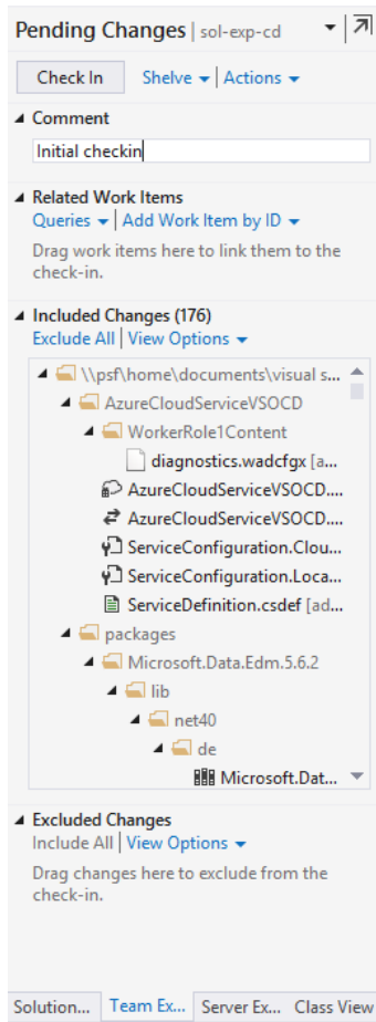
FIGURE 3-15 The Pending Changes pane of Team Explorer
