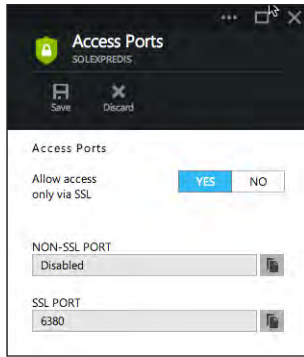
FIGURE 5-29 Setting access ports for a Redis cache
