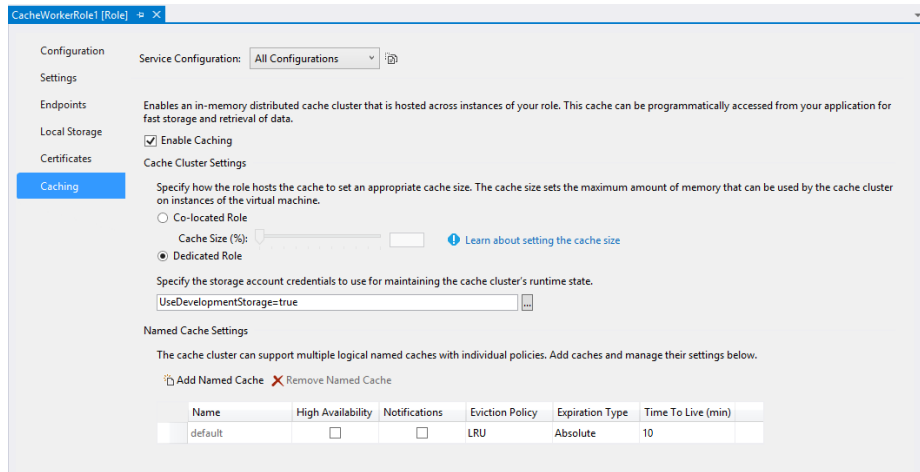
FIGURE 3-12 The caching tab in Visual Studio
