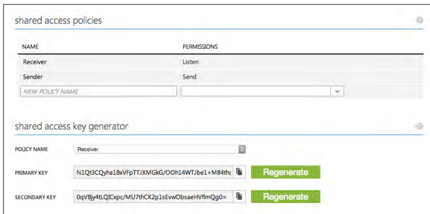
FIGURE 5-17 Managing keys for shared access policies
