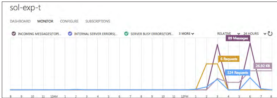
FIGURE 5-23 The metrics graph presented on the Monitor tab for a topic
