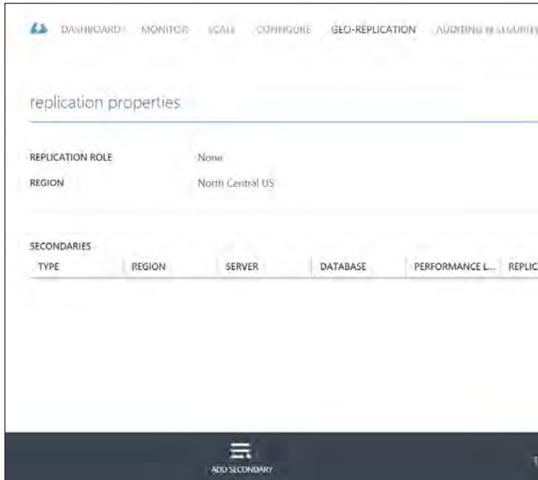
FIGURE 4-16 Replication properties
