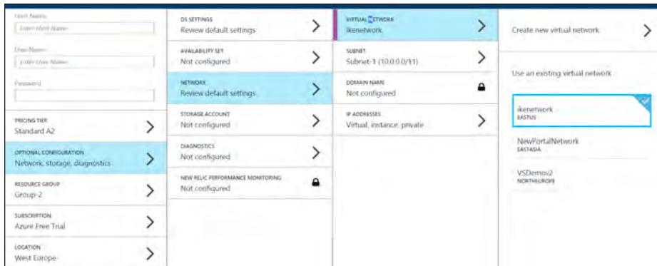
FIGURE 5-11 Selecting an existing virtual network for a new VM
