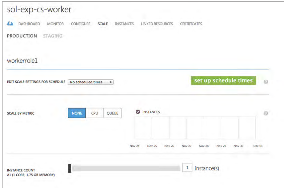
FIGURE 3-5 The scale tab for a cloud service in the management portal
