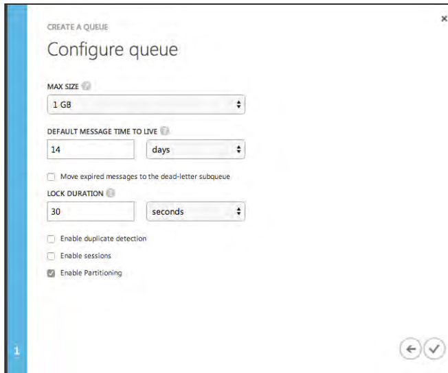
FIGURE 5-19 Additional setting available when creating a new queue
