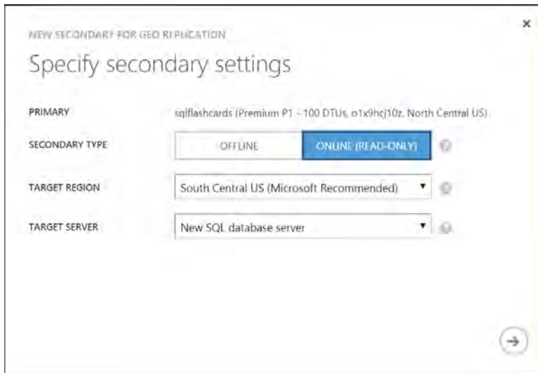
FIGURE 4-19 The New Secondary For Geo Replication dialog box for creating an active secondary
