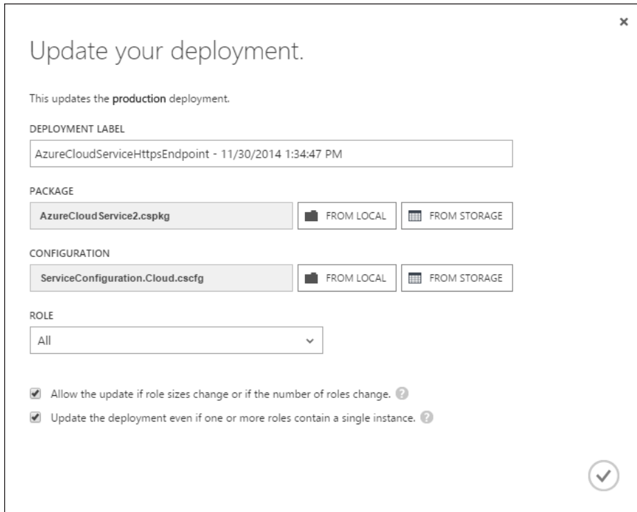
FIGURE 3-14 The Update Your Deployment screen
