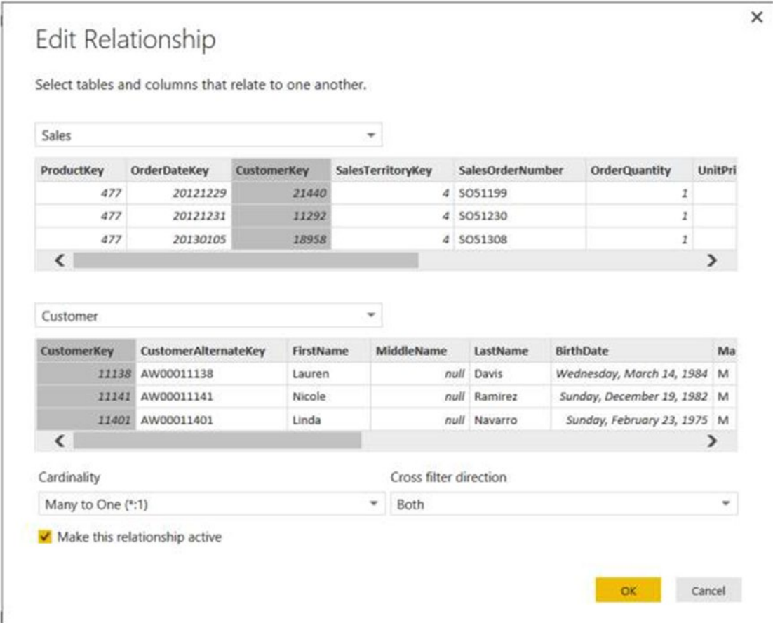
Figure 9-15. Editing a table relationship
