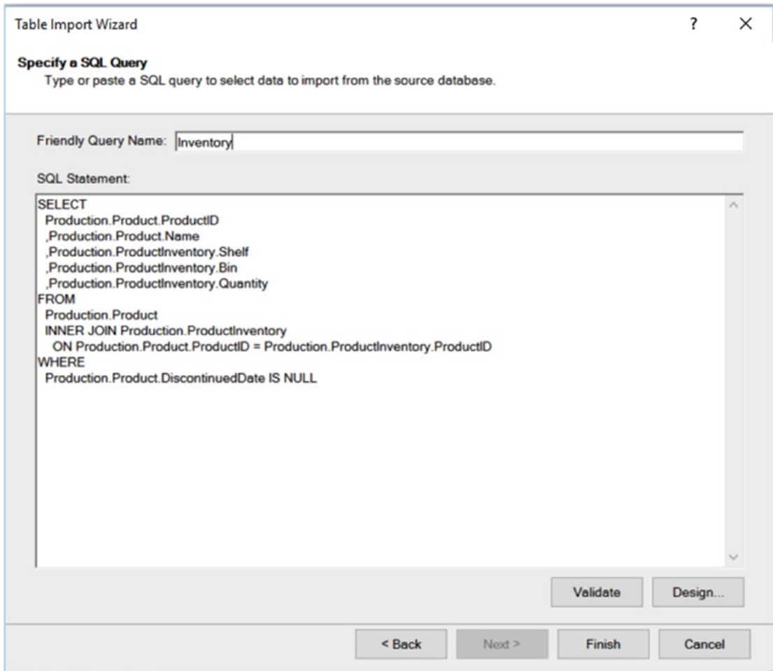
Figure 2-16. Viewing and validating the query
