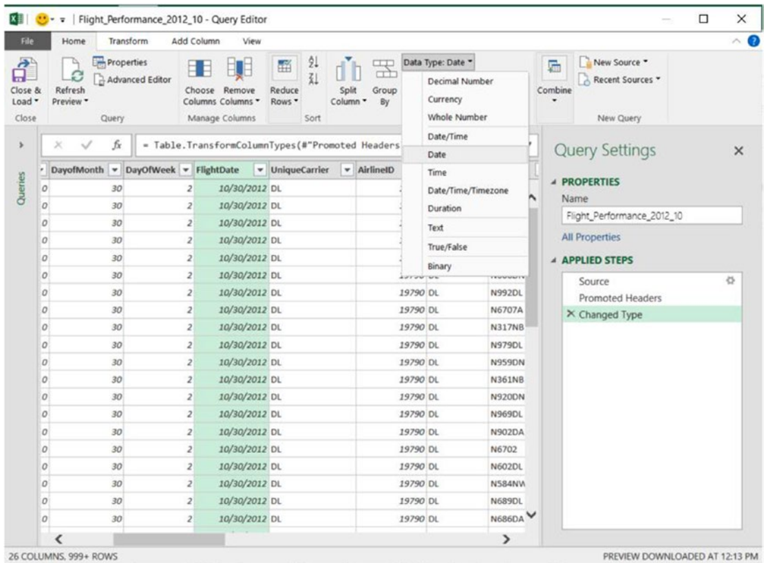
Figure 3-5. Changing the data type of a column
