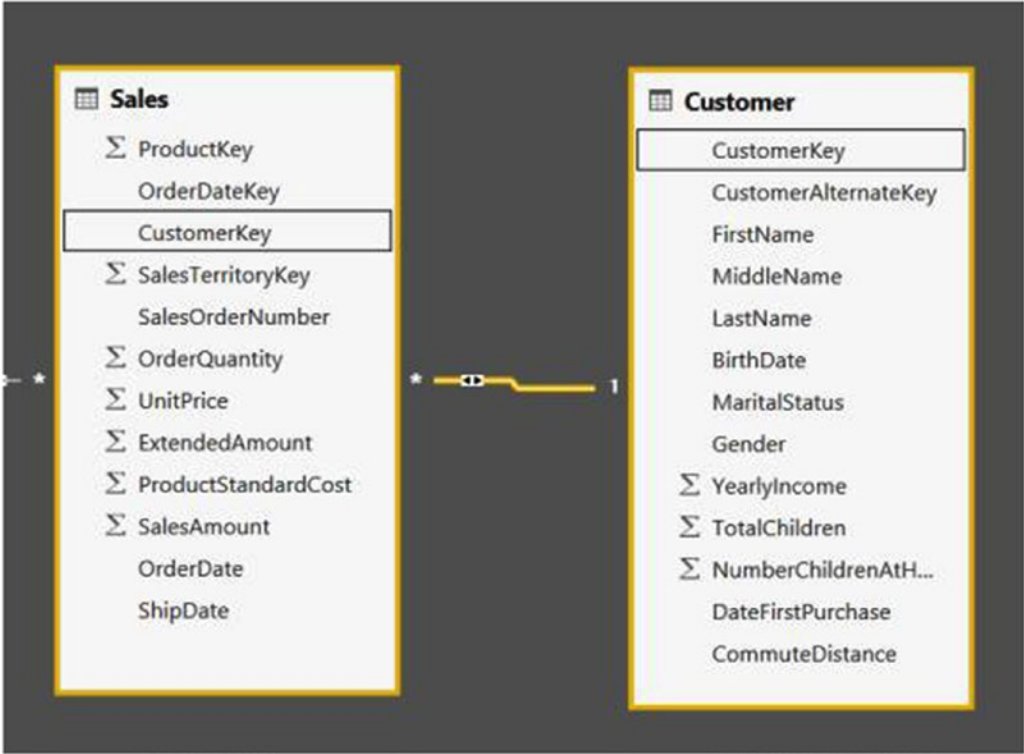
Figure 9-16. Viewing a relationship in the Relationship view
