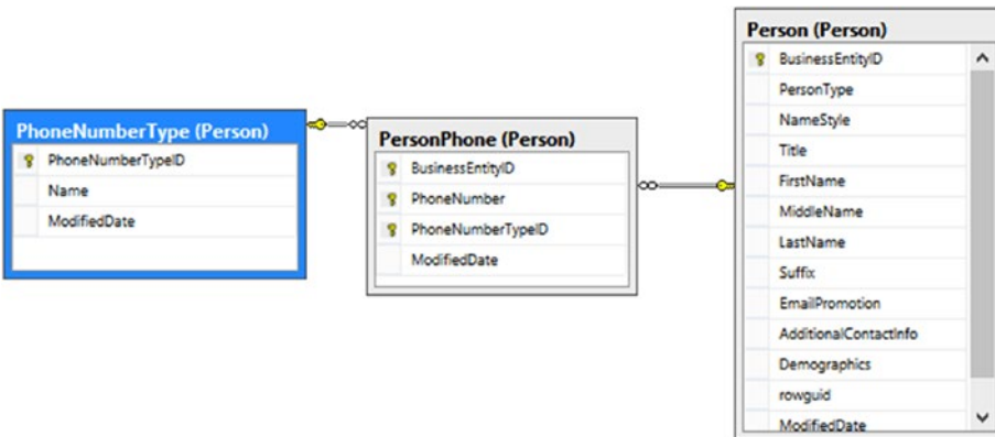
Figure 2-2. A many-to-many relationship
