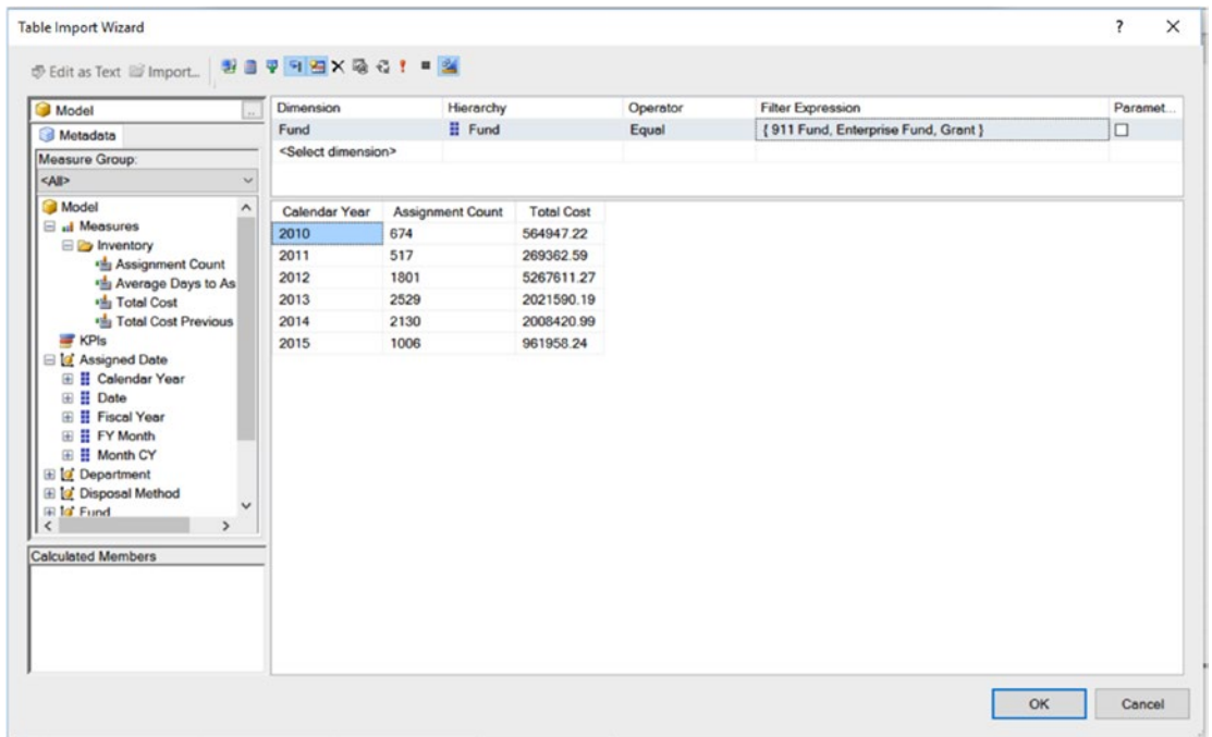
Figure 2-25. Designing an MDX query
