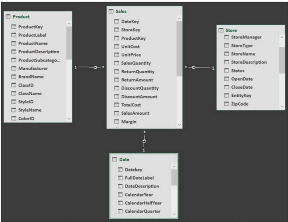
Figure 4-10. A typical star schema
