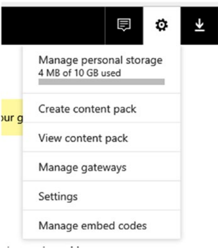
Figure 11-25. Managing gateways
